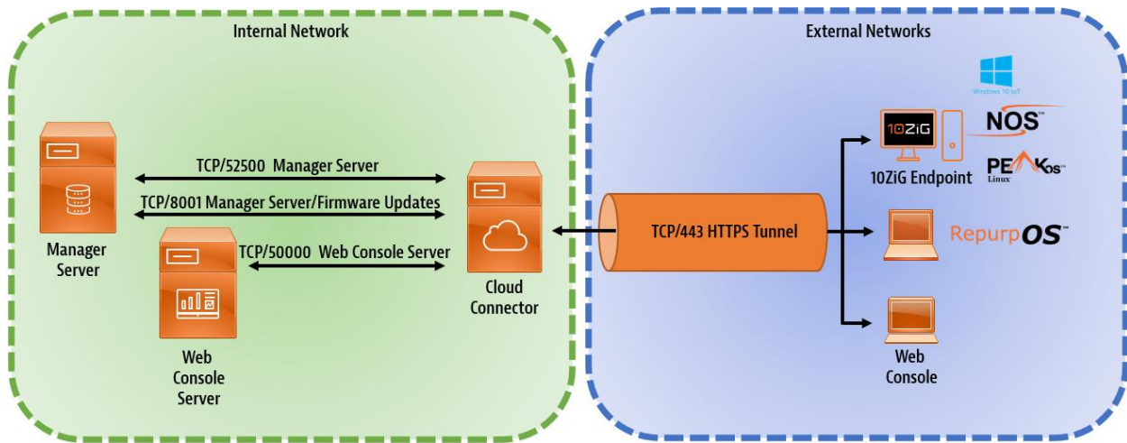
FIGURE 3 MANAGEMENT PROTOCOLS COMMUNICATION CHANNELS WITH SECURE CONNECTOR IN USE .
