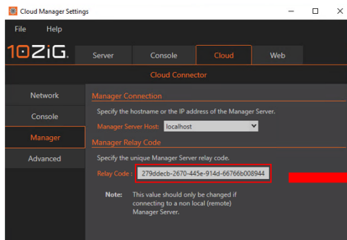
Manager Server
