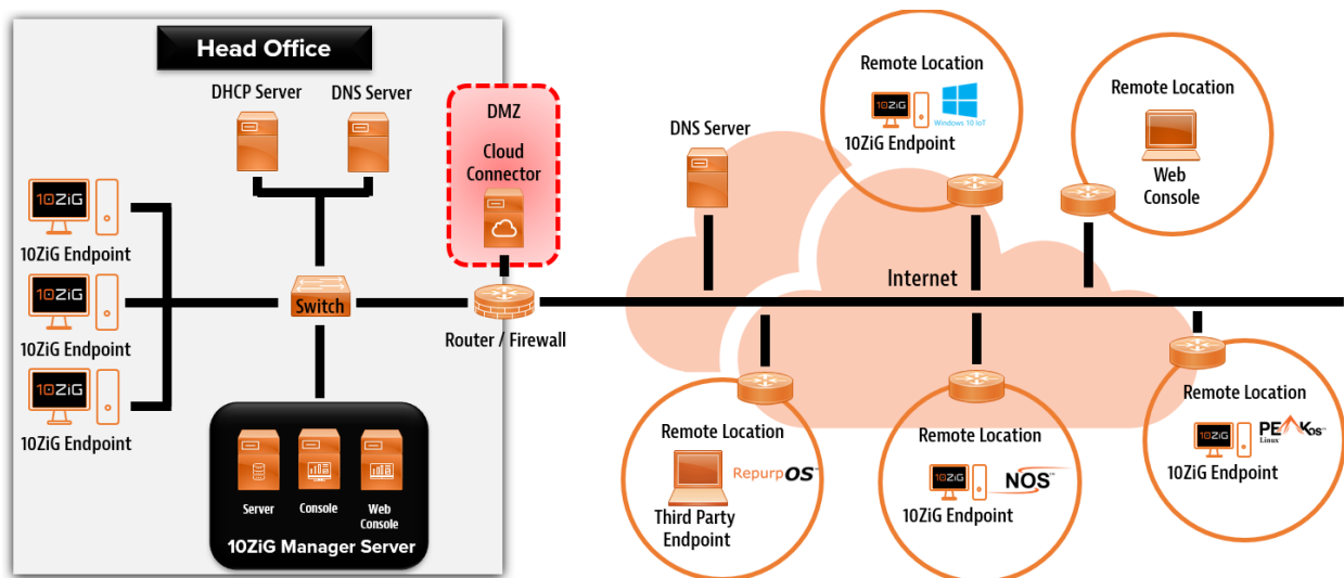
FIGURE 7 DEPLOYMENT SCENARIO 2 EXAMPLE NETWORK DIAGRAM
