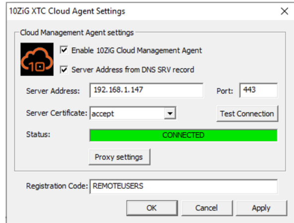
Windows 10 IoT
