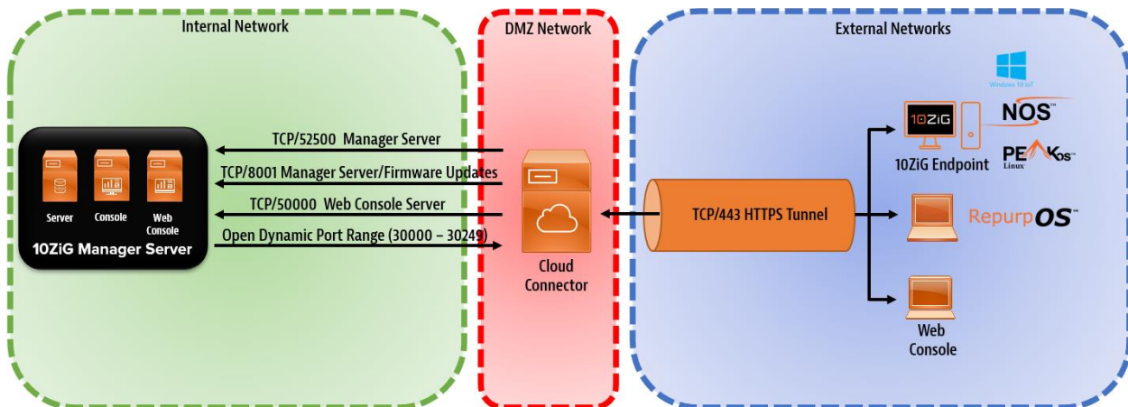
FIGURE 5 INTERNAL 10ZiG MANAGER SERVER AND DMZ BASED SECURE CONNECTOR ACCESSIBLE EXTERNALLY
